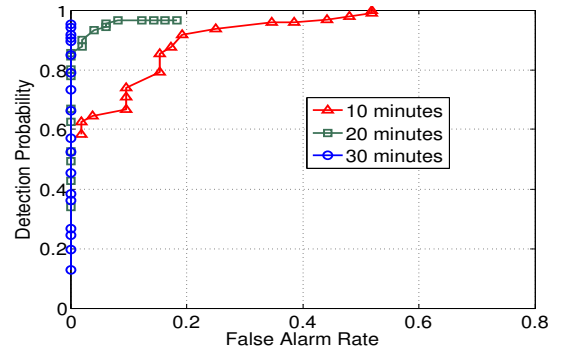
Fig. 6. ROC for audio recapture detection with different clip length.
